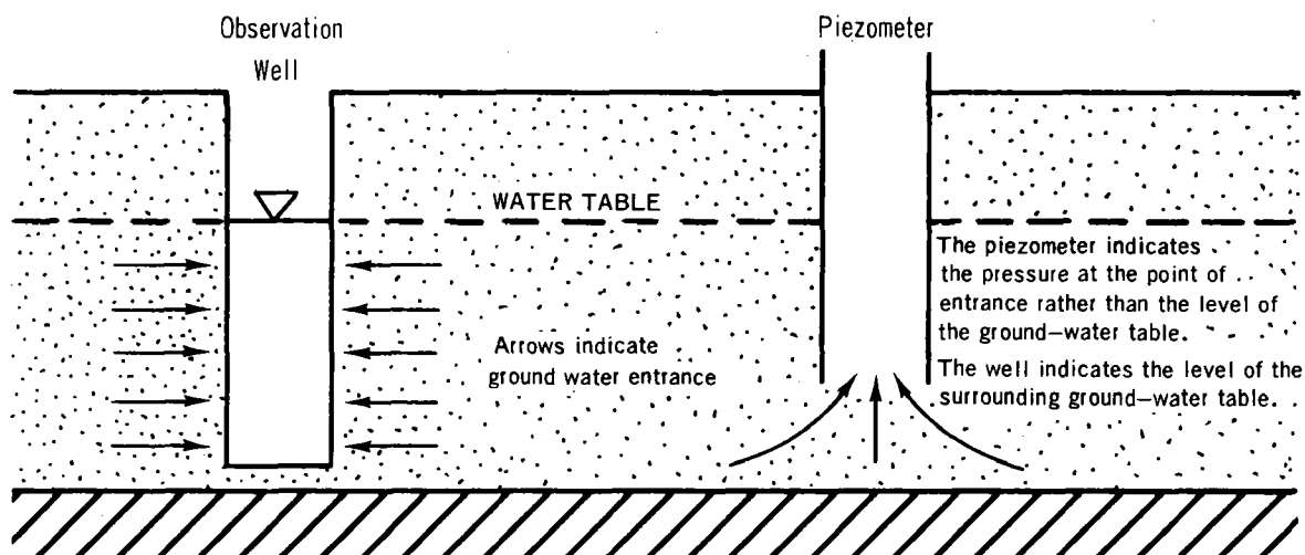
A – Construction of observation wells and piezometers
