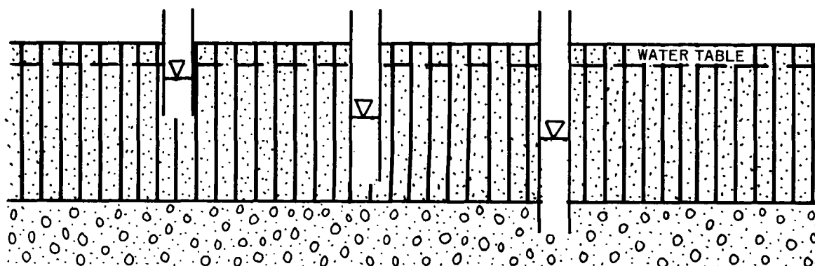
C – Piezometers indicate a perched water table draining slowly into underlying sand and gravel.
