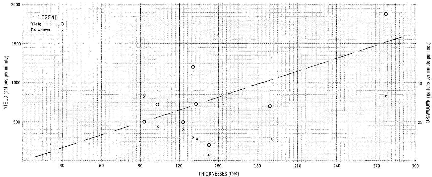
FIGURE 2-3 Yields of Saturated Very-fine Sands in Wells (Compiled from Cady and Scherer, 1946)
