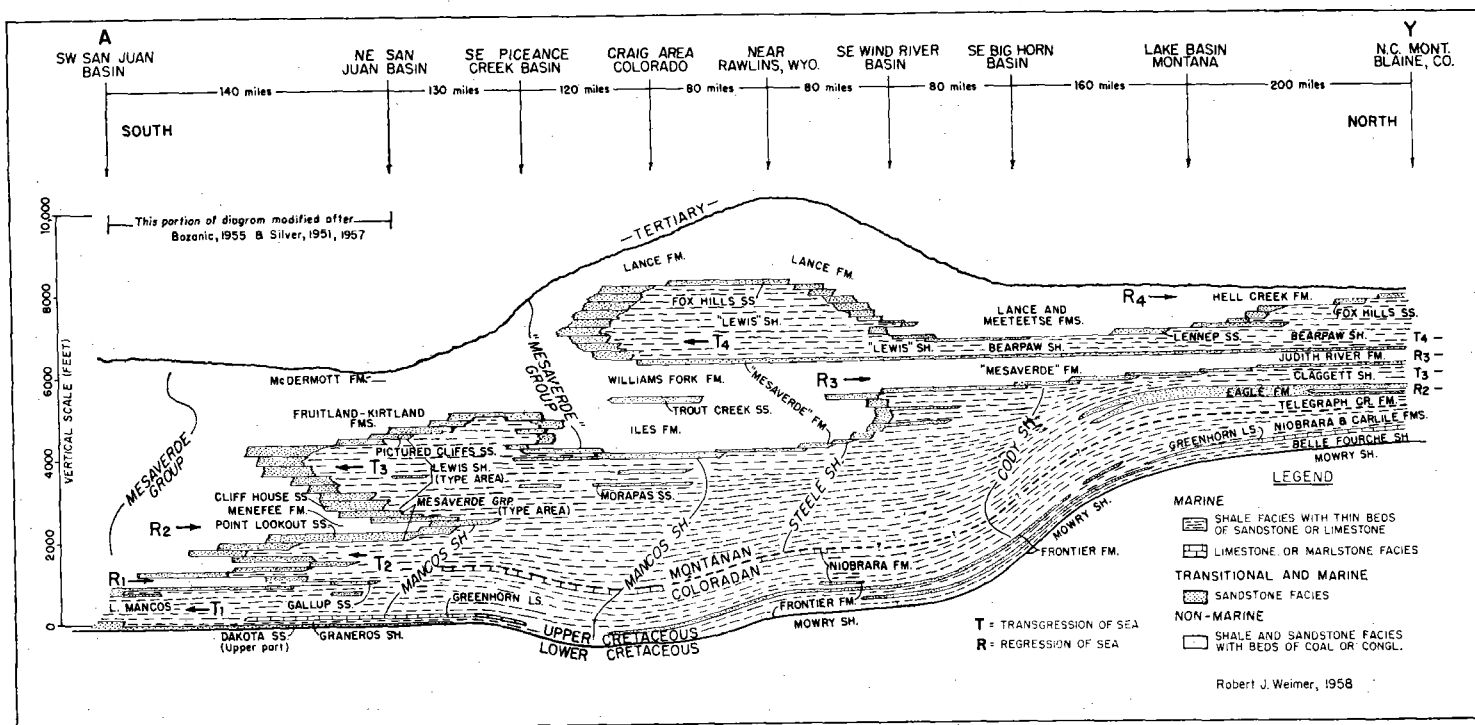
FIGURE 2-6. Stratigraphic diagram of Western U. S.
