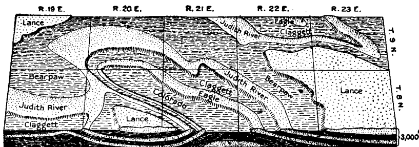
FIGURE 2-11. Stereogram of central Montana
