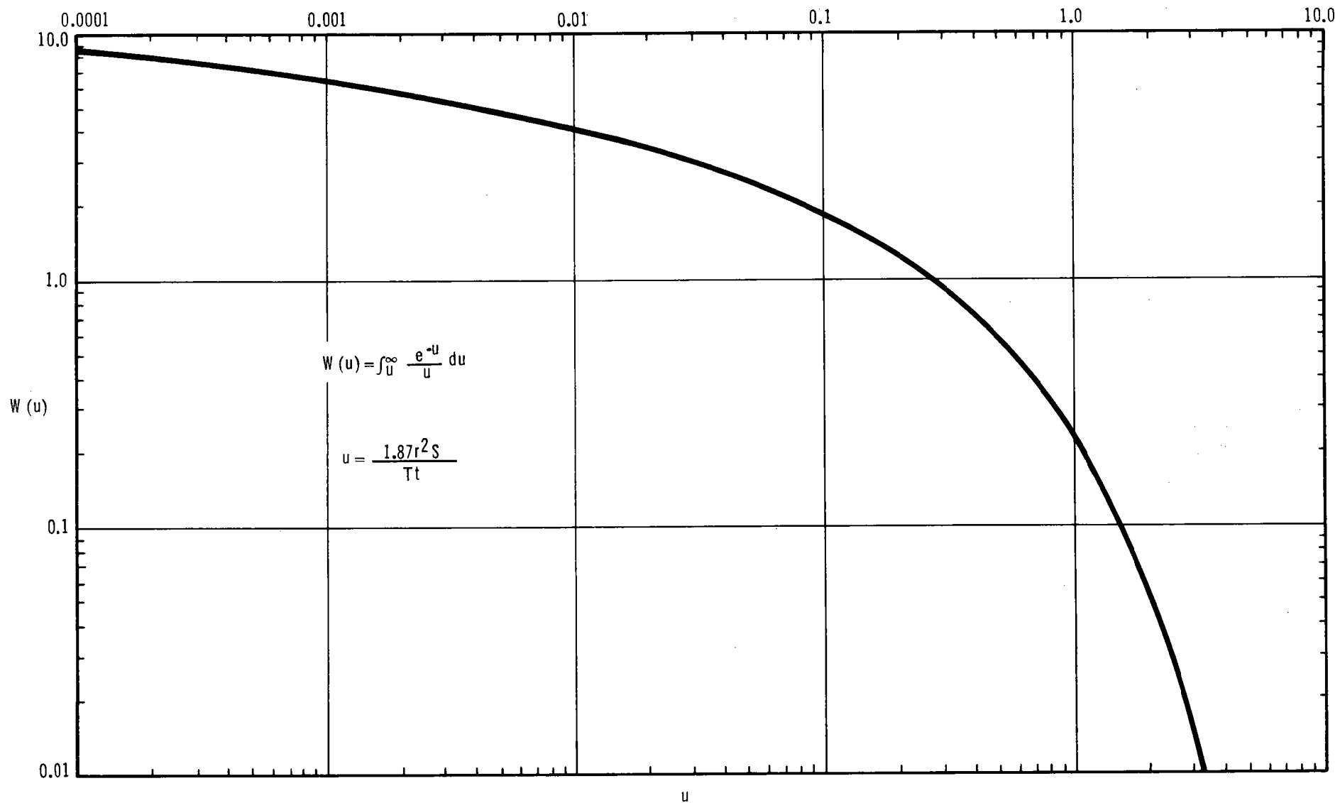
FIGURE 1 - 8 Relation Between u and W(u)
