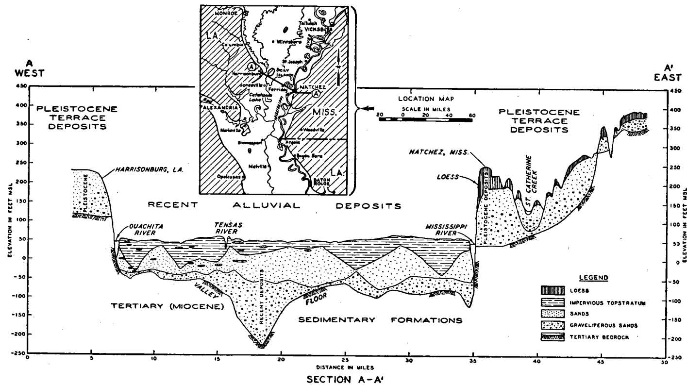
FIGURE 2-1. Geological section near Natchez, Mississippi
