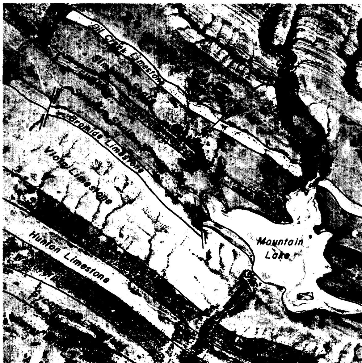
FIGURE 4-2 Aerial photograph used in geologic mapping
