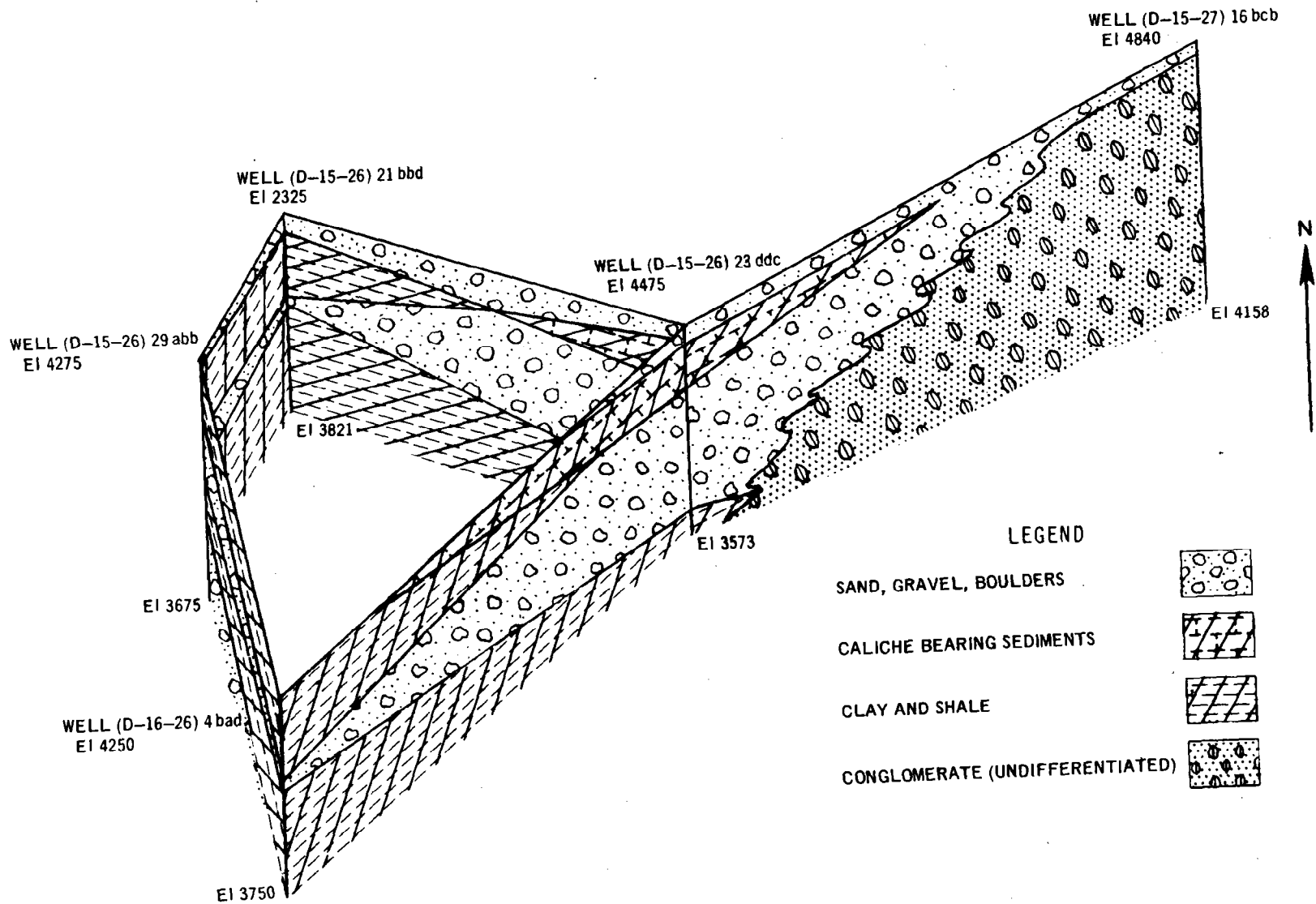
FIGURE 4-5. Fence Diagram
