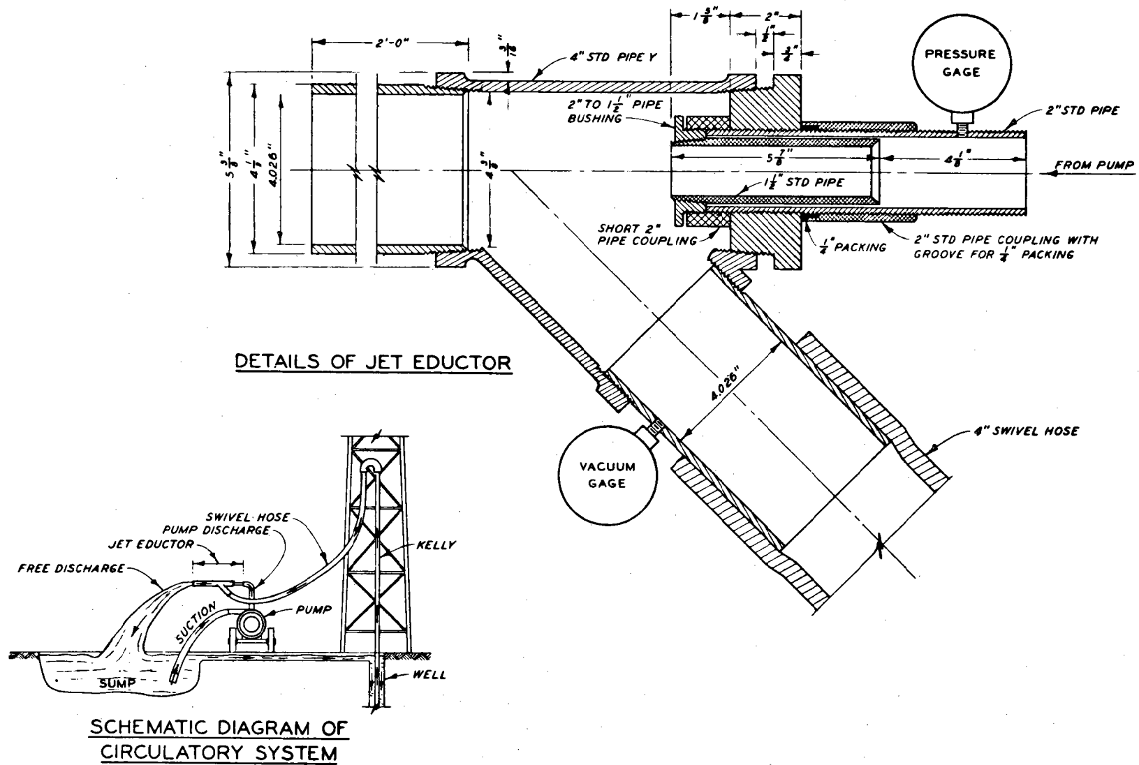
Figure 6-1. Reverse Circulation Drilling
