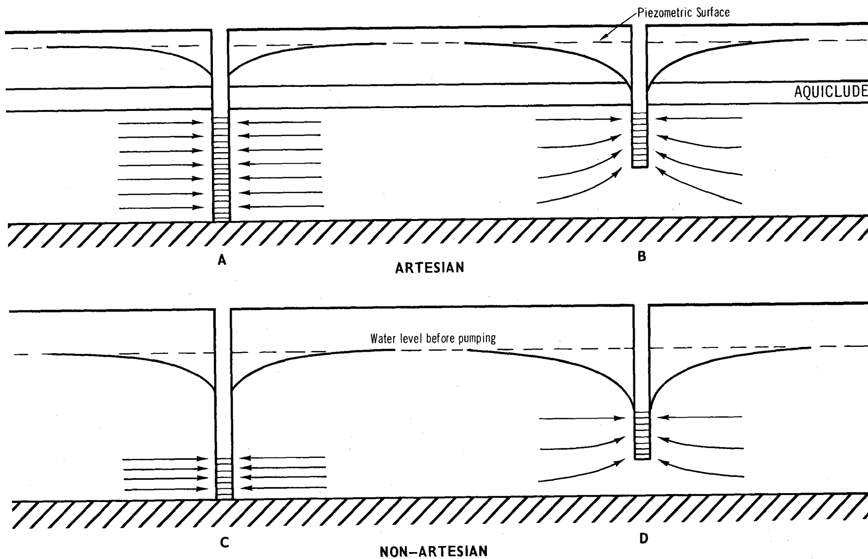
Figure 6-8. Full and Partial Penetration of Wells
