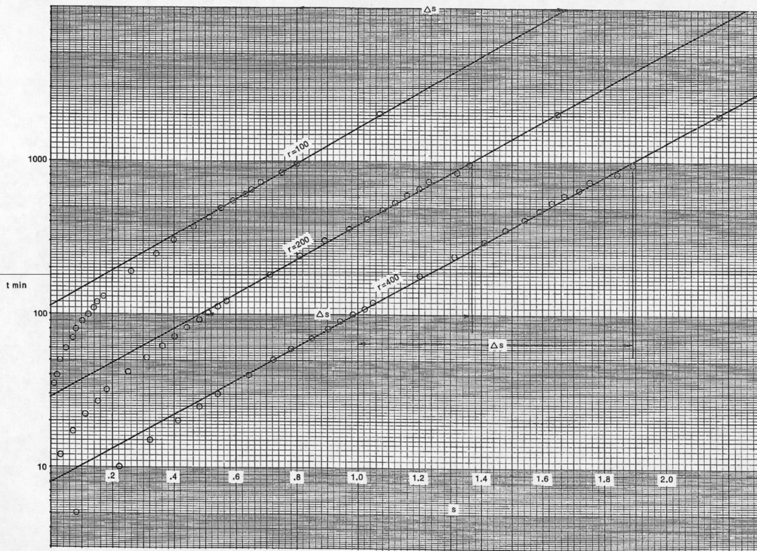
FIGURE 3-12. Time Drawdown Curves
