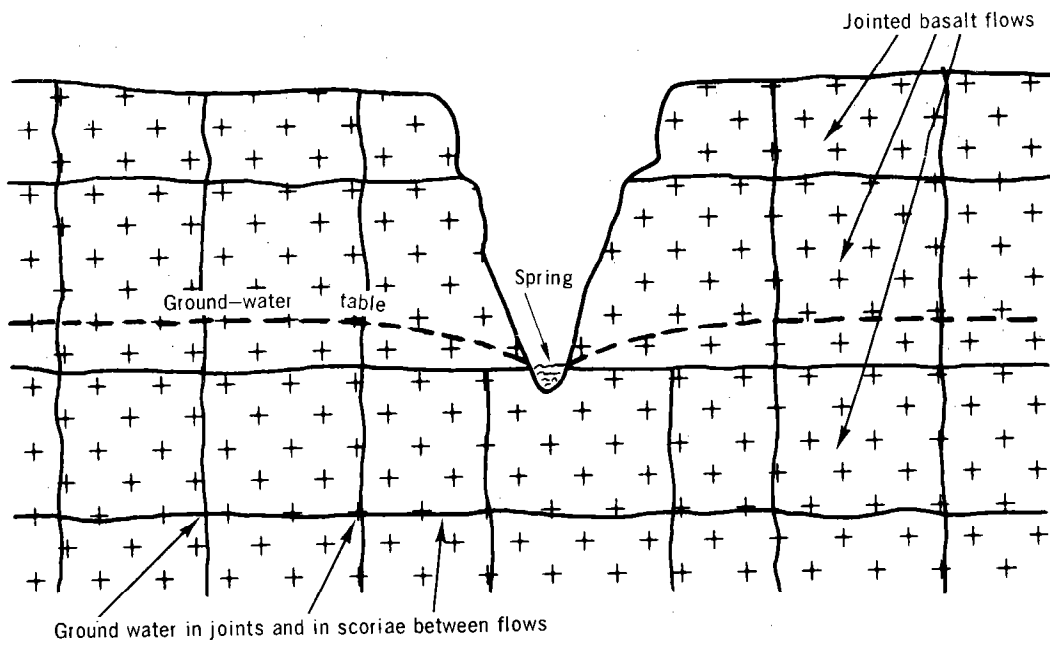
Figure 5-4. Spring in Jointed Basalt
