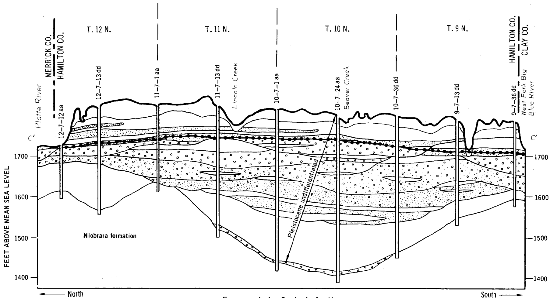
FIGURE 4-4 Geologic Section
