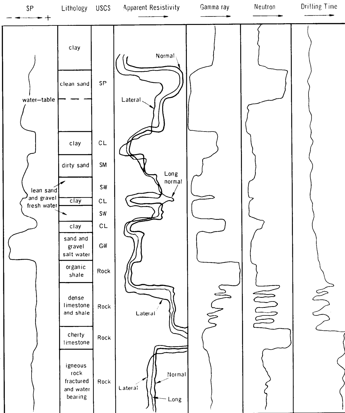
FIGURE 6-7. Examples of Well Logs
