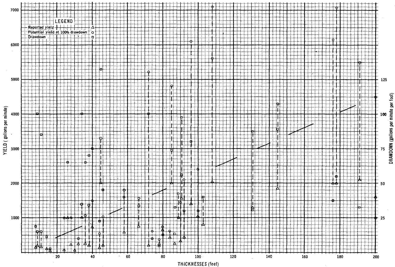
FIGURE 2-4 Yields and Potential Yields of Saturated Sands and Gravels in Irrigation Wells
