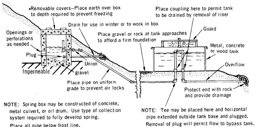
SECTIONAL ELEVATION
