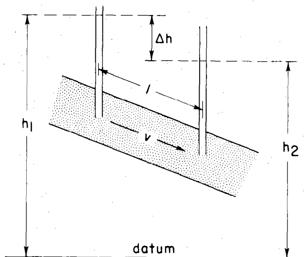
FIGURE 1-3. - Factors involved in Darcy's Law
