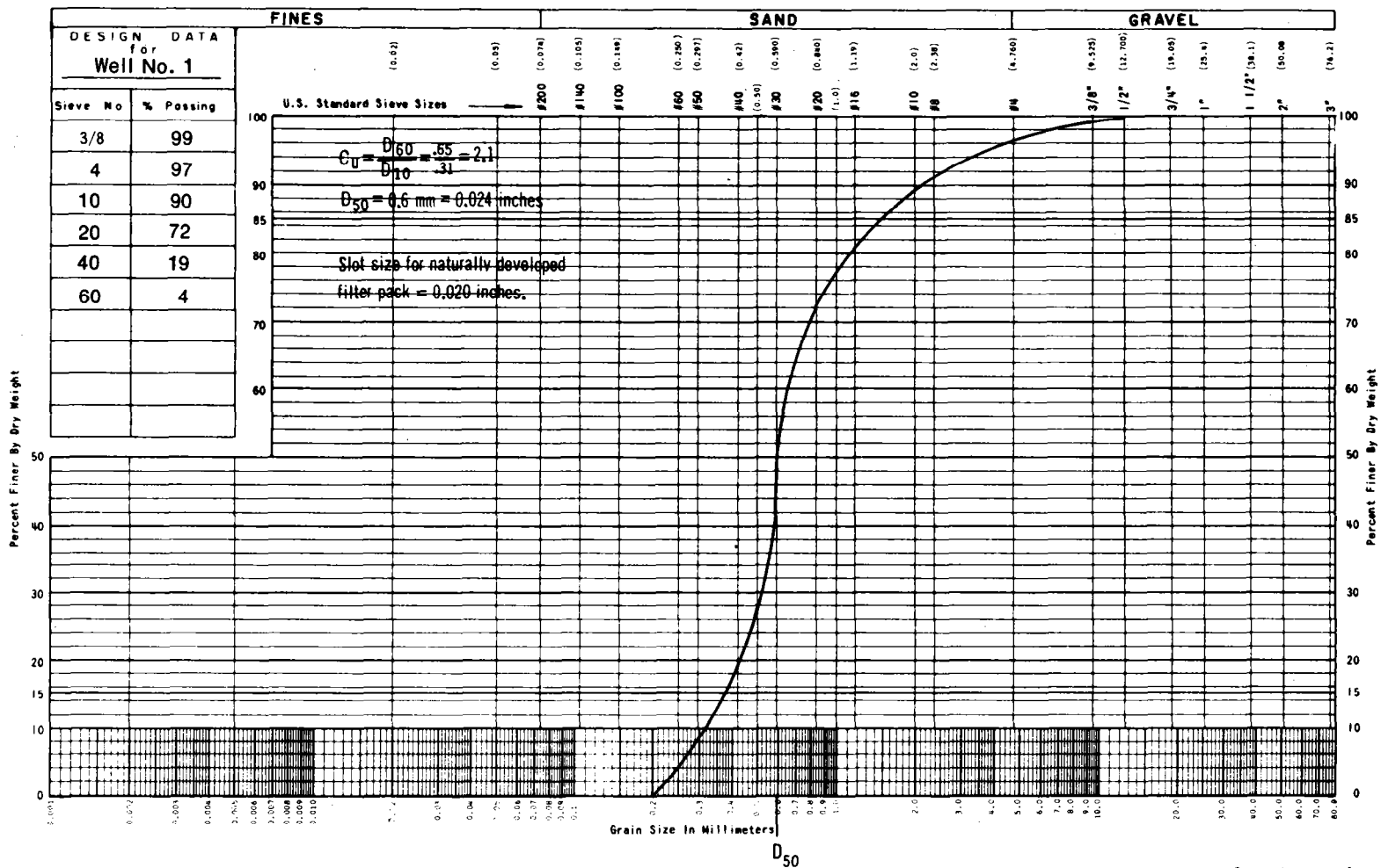
FIGURE 6-10. Natural Filter Pack Design
