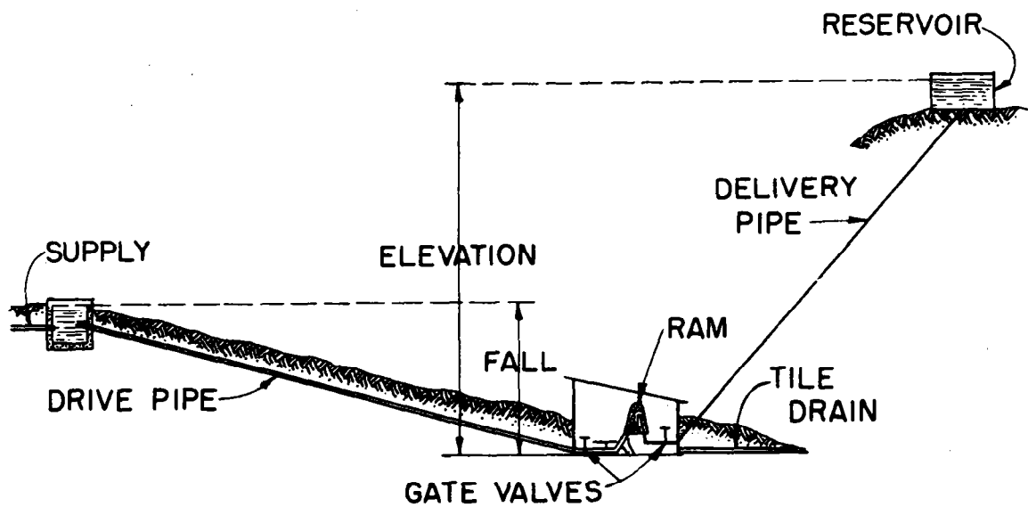
SKETCH OF TYPICAL RAM INSTALLATION
