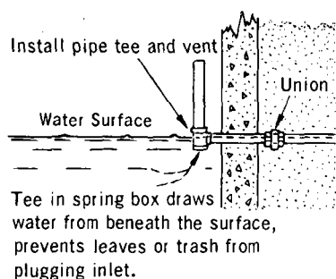
DETAIL-DELIVERY PIPE INLET
