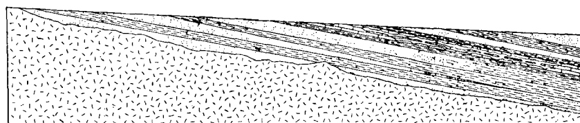
FIGURE 2-9. Stratigraphic traps
