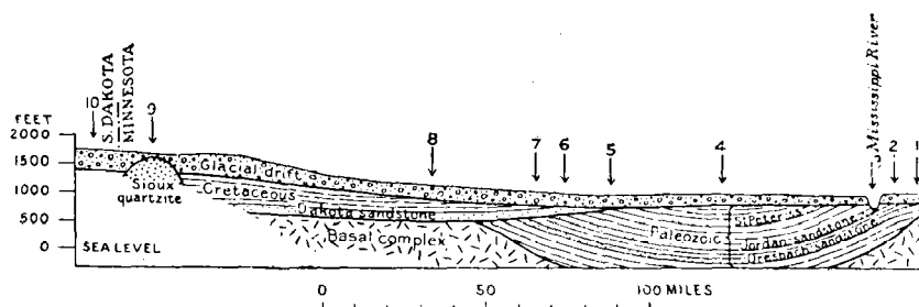
FIGURE 2-8 Stratigraphic traps
