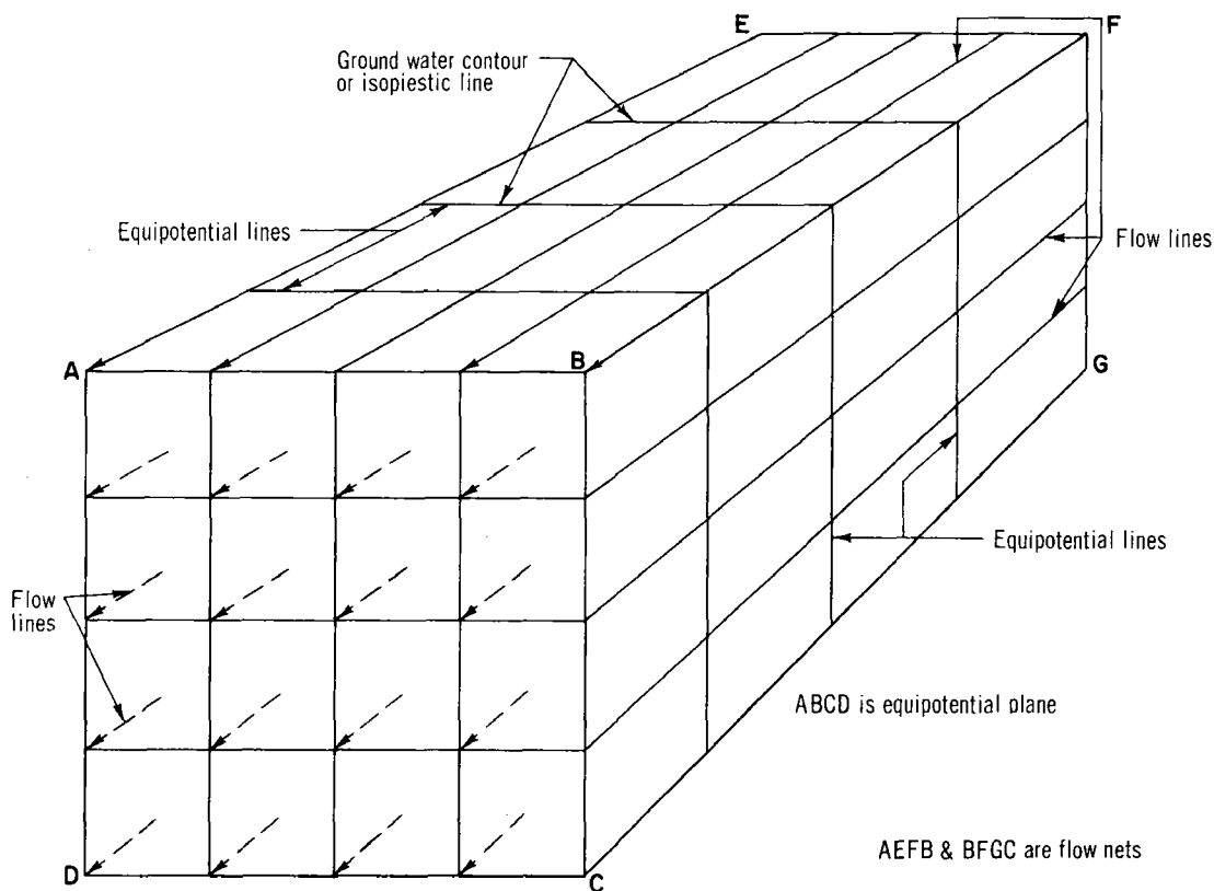
Figure 1-5. Flow Nets
