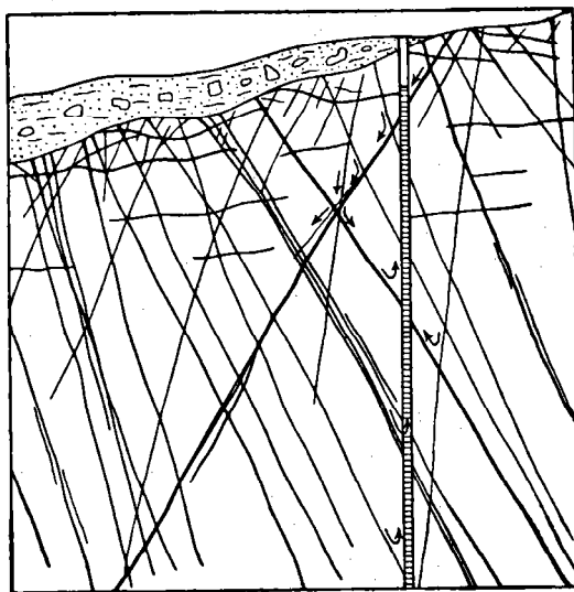
FIGURE 2-12. Joint system
