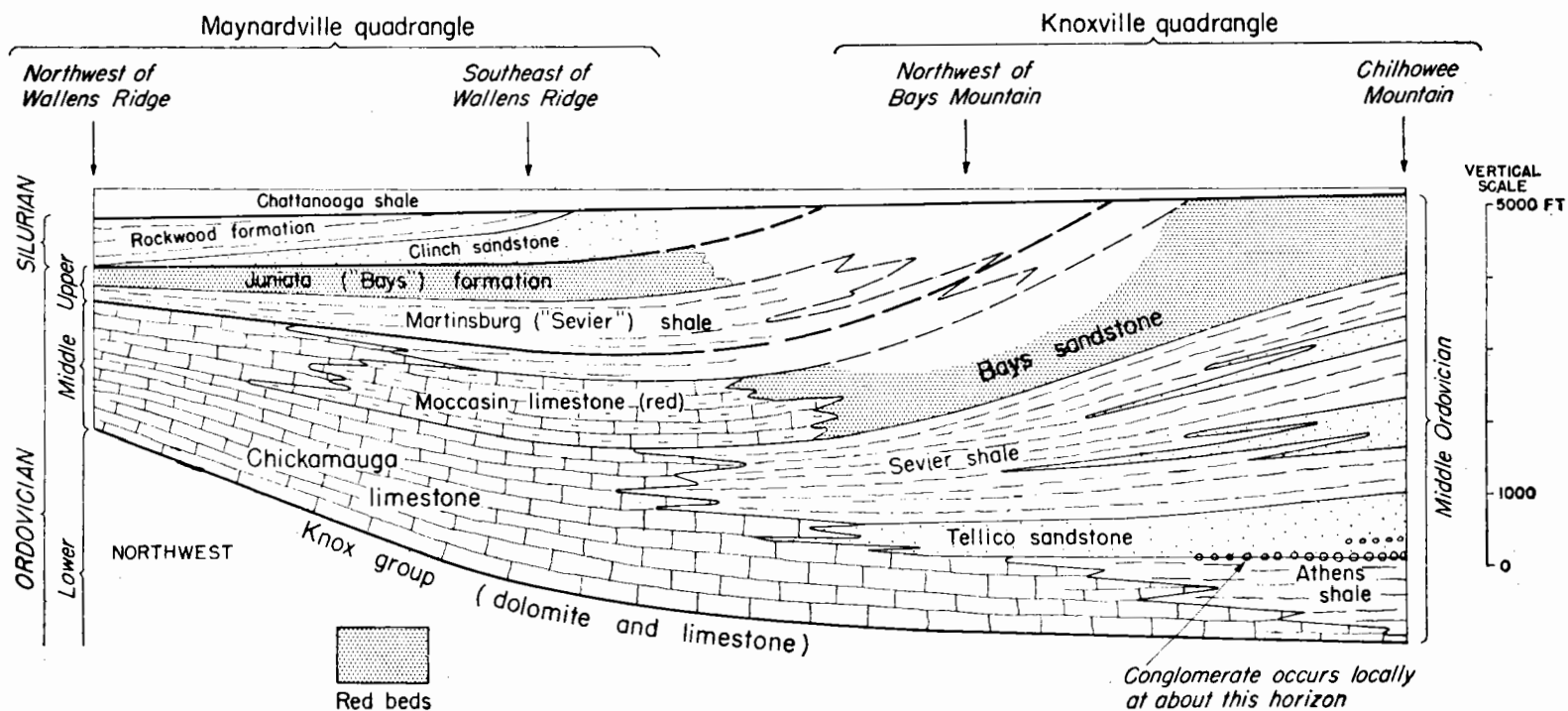
FIGURE 2-7. Stratigraphic diagram of Tennessee
