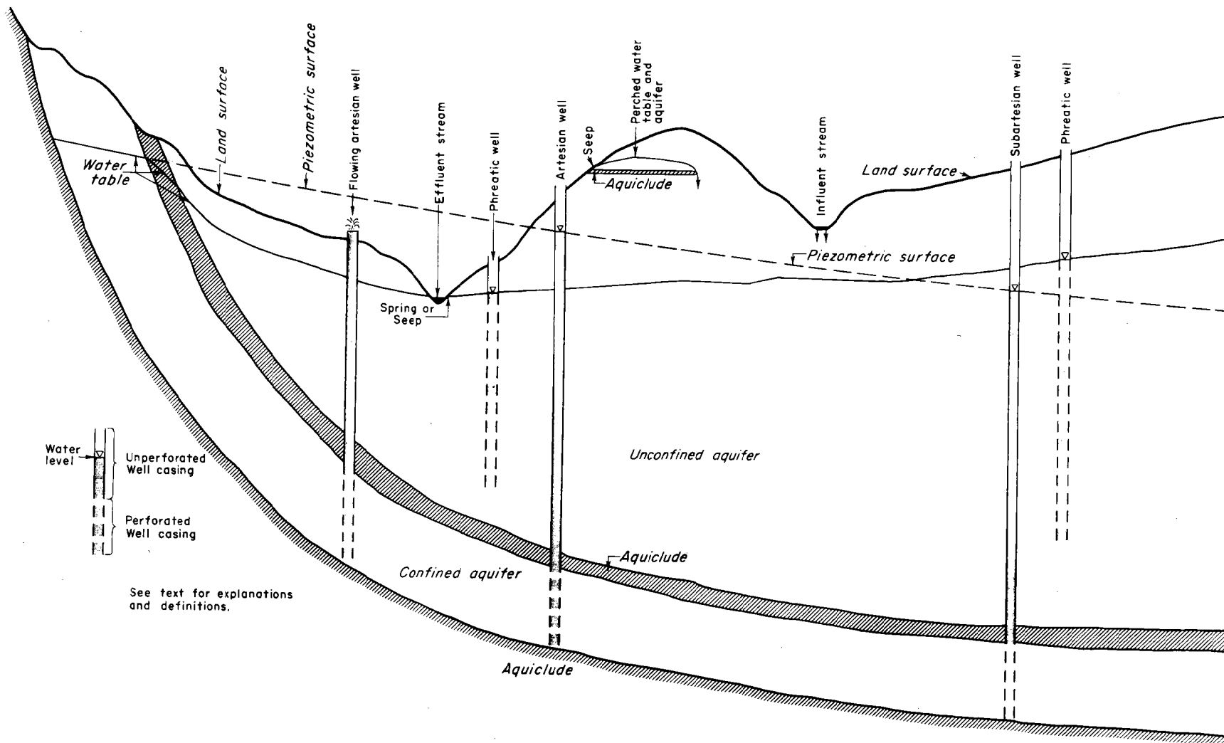
Figure 1-2. Ground-water Relationships
