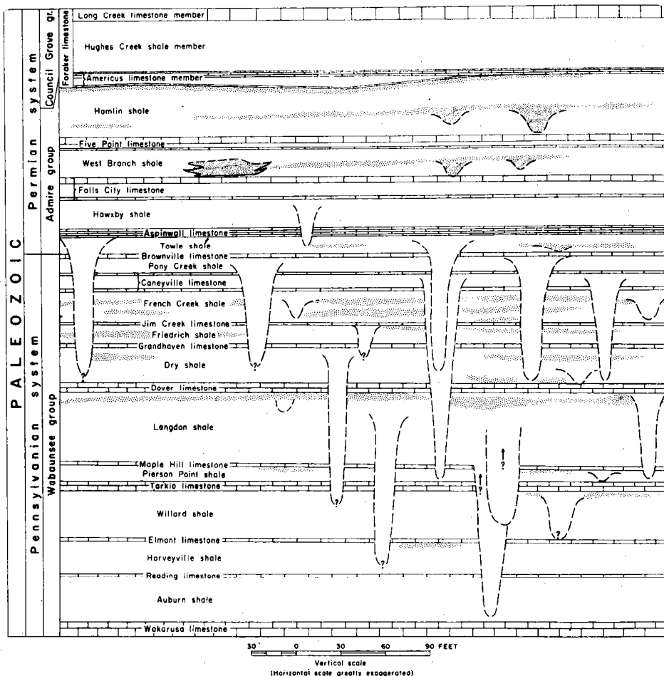
FIGURE 2-10. Buried channels
