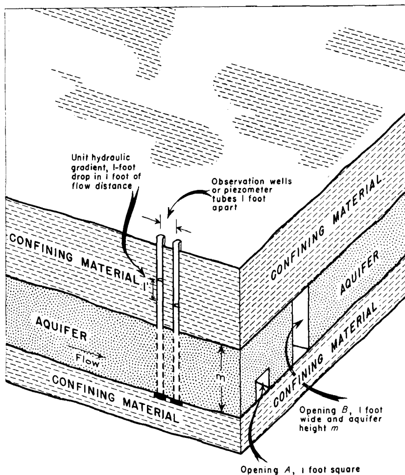
Figure 1-4. Coefficients of Permeability and Transmissibility
