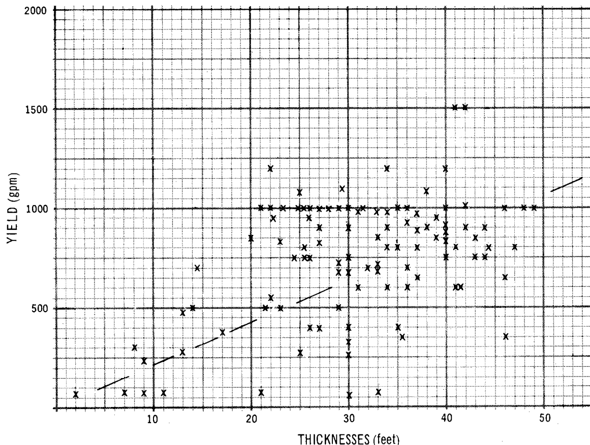
FIGURE 2-2 Yields of Saturated Sands and Gravels in Irrigation Wells
