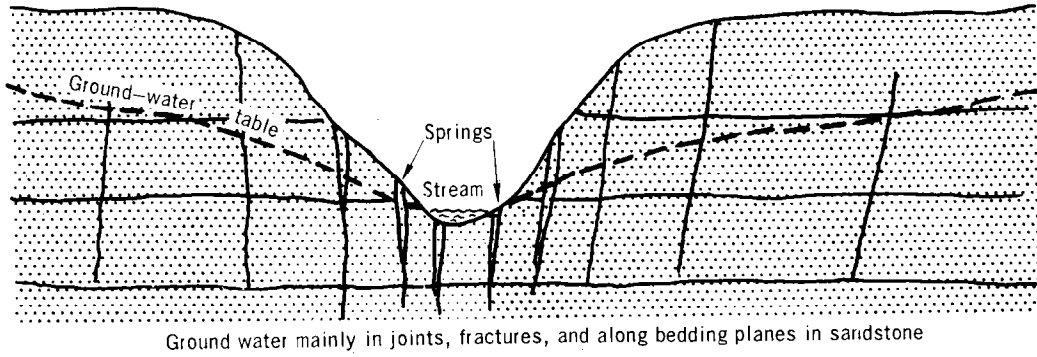
Figure 5-3. Spring in Jointed Sandstone
