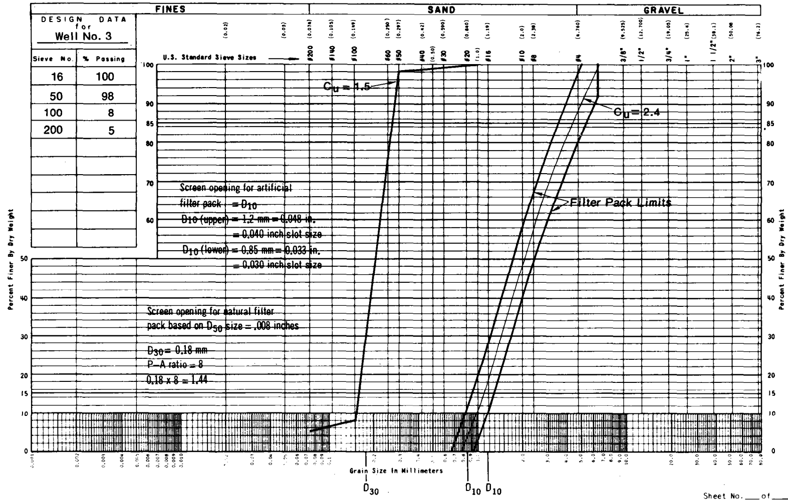
FIGURE 6-13. Artificial Filter Pack Design
