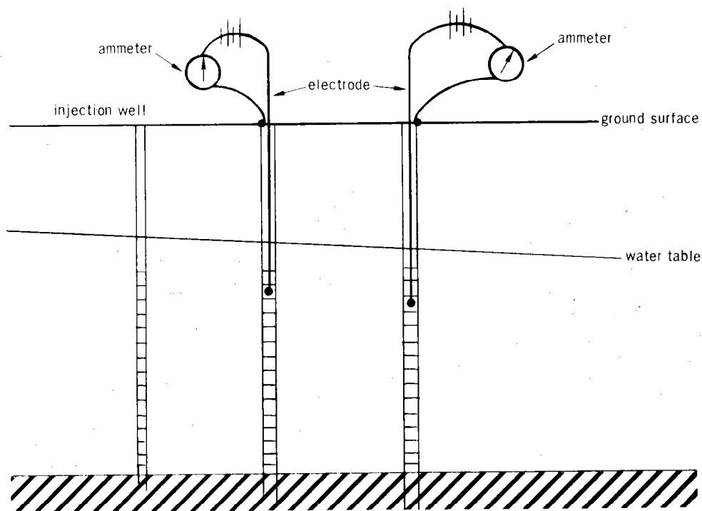
FIGURE 4-3. Typical salt detection arrangement
