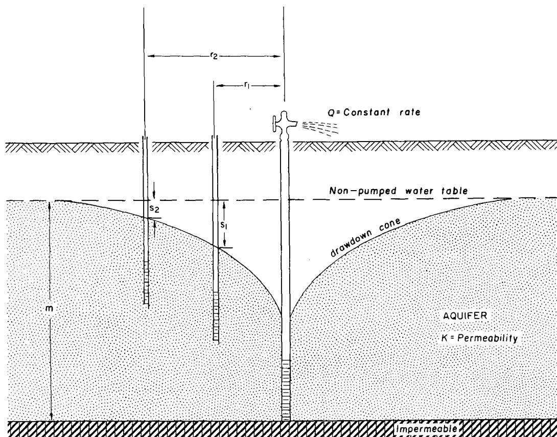
Figure 1-7. Aquifer Pump Test
