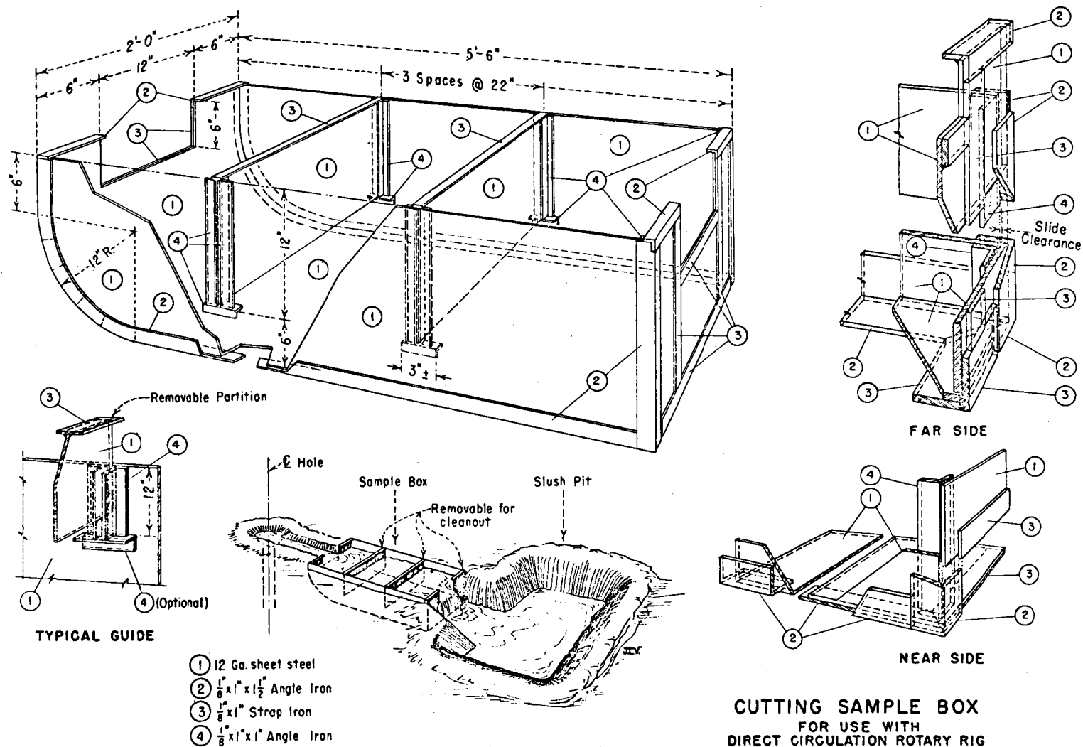
Figure 6-2. Cutting Sample Box
