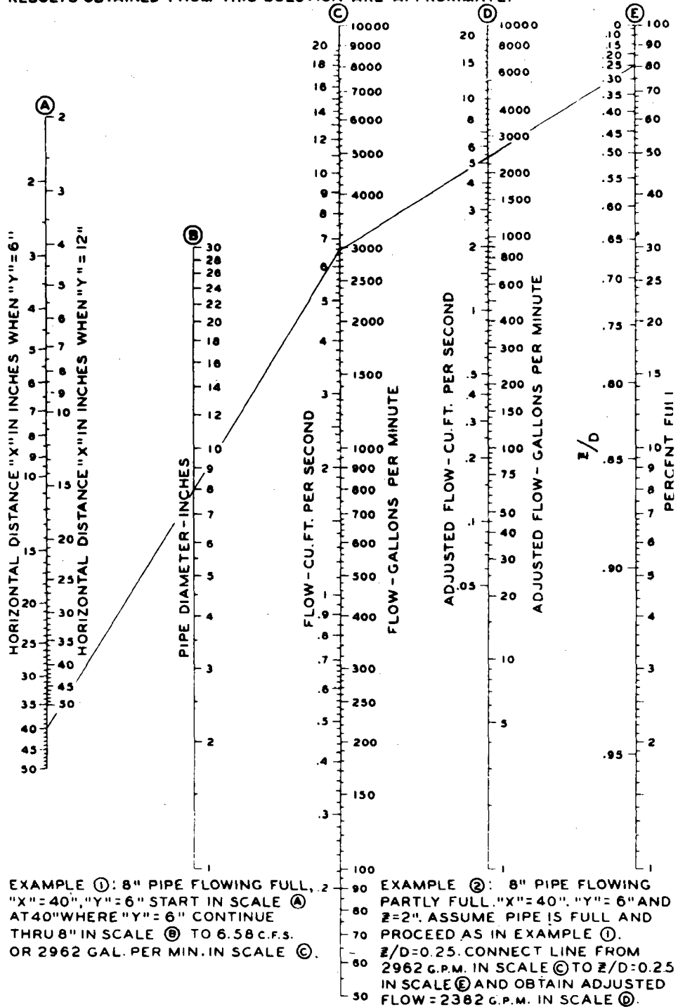
Figure 3-3. Estimated Flows from Pipes
