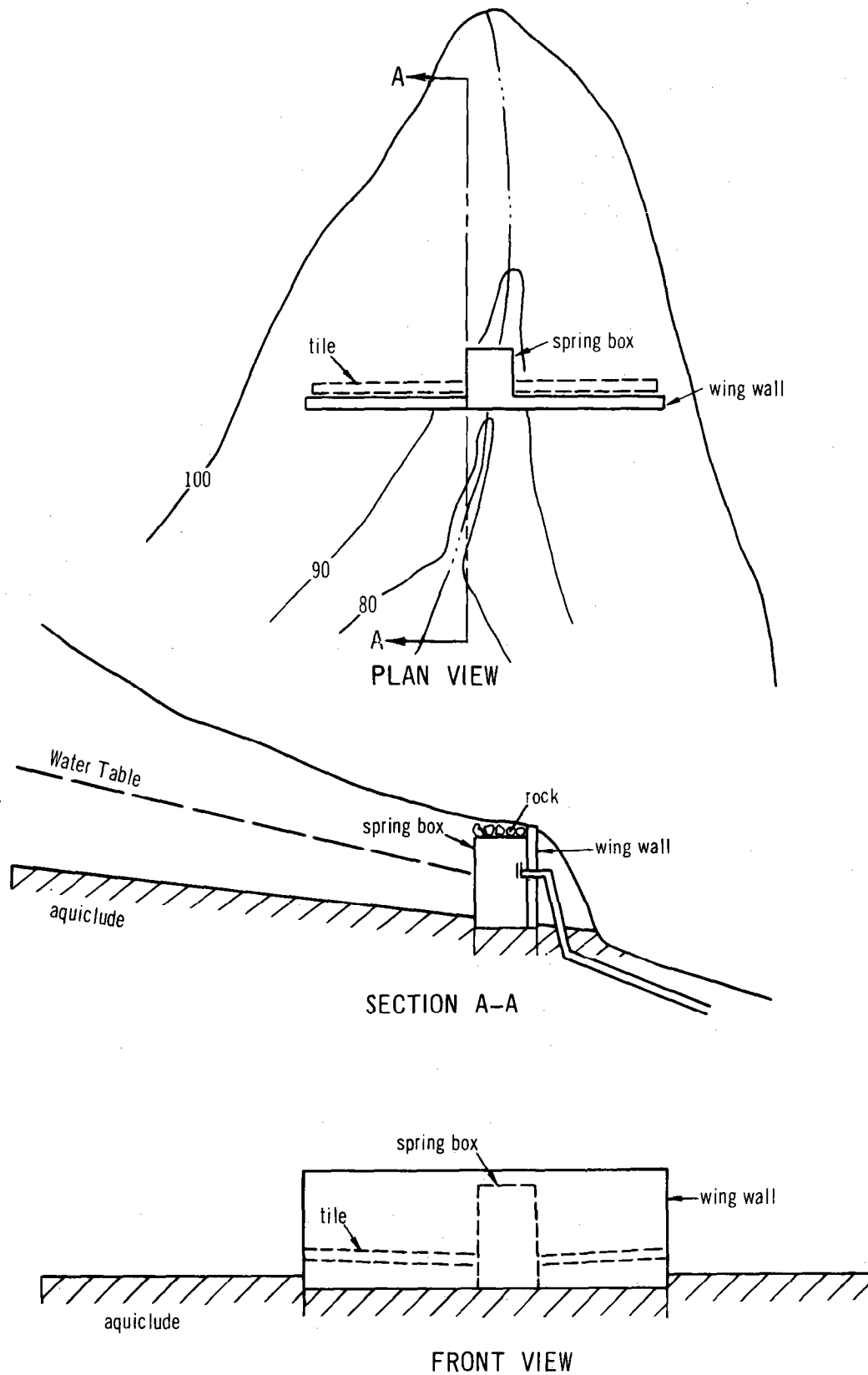
Figure 5-11. Spring Development in Stream Channel
