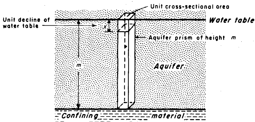
B. WATER-TABLE AQUIFER
