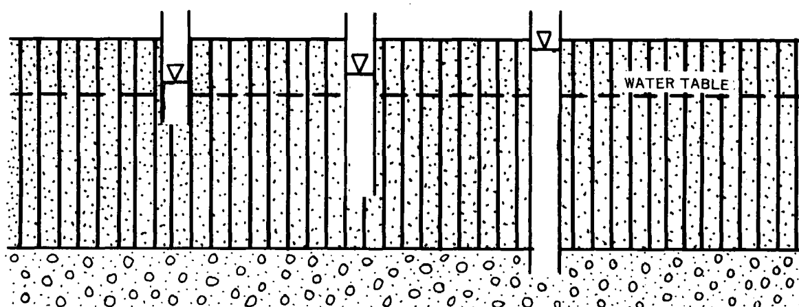
B – Piezometers indicate water under artesian pressure in sand and gravel zone is leaking into overlying material.
