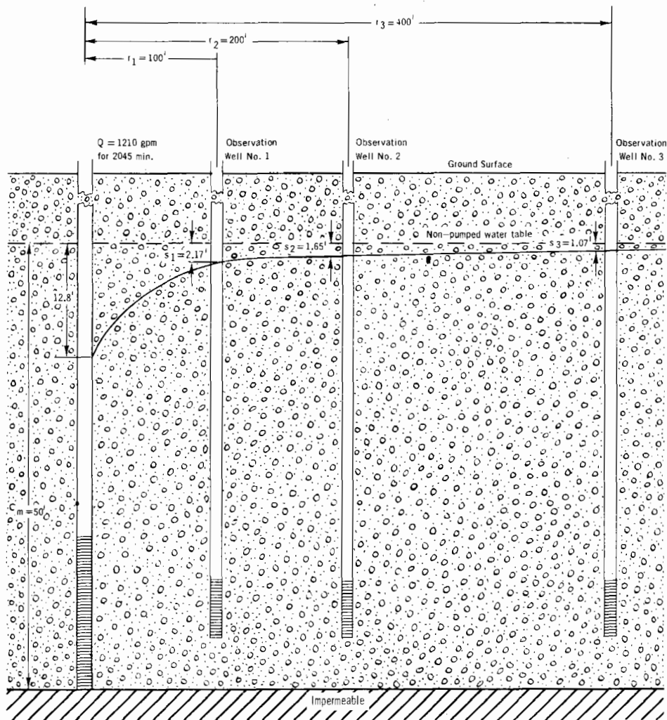
Figure 3-8. Drawdown Cone
