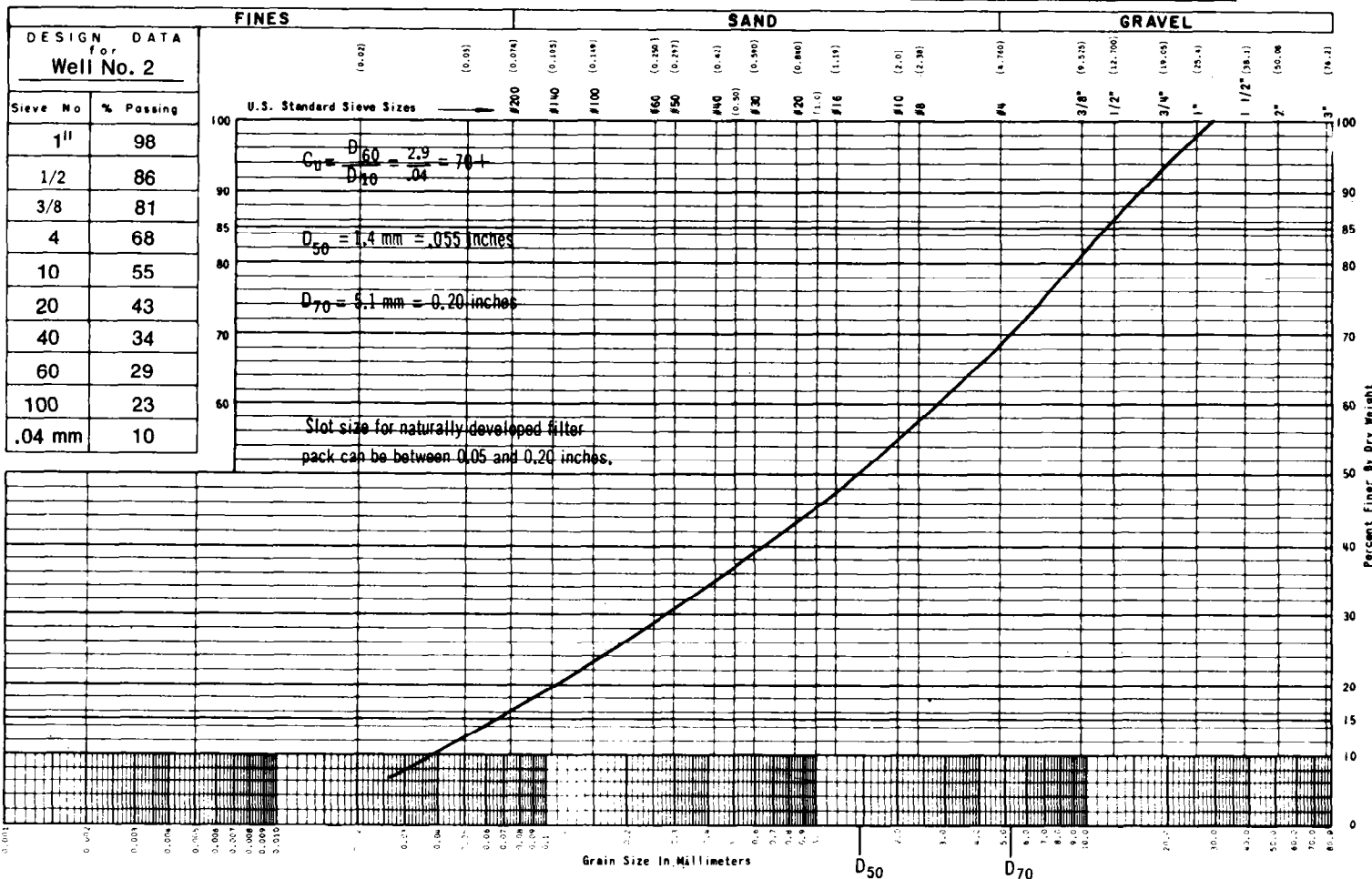
FIGURE 6-11. Natural Filter Pack Design
