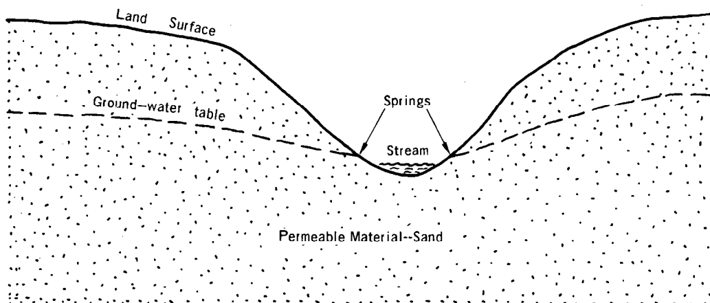
Figure 5-1. Depression Spring, Seepage or Filtration Type
